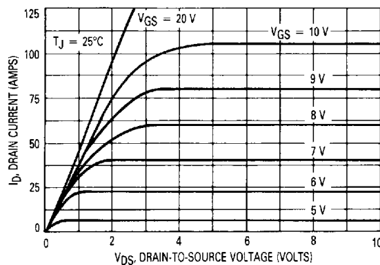
FIGURE 2 — ON-REGION CHARACTERISTICS
