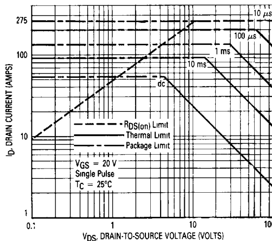
FIGURE 13 — MTM55N10
