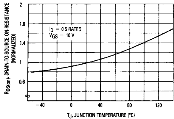
FIGURE 10 — ON-RESISTANCE VARIATION WITH TEMPERATURE
