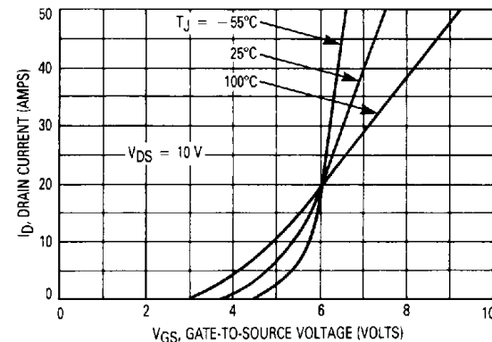
FIGURE 4 — TRANSFER CHARACTERISTICS
