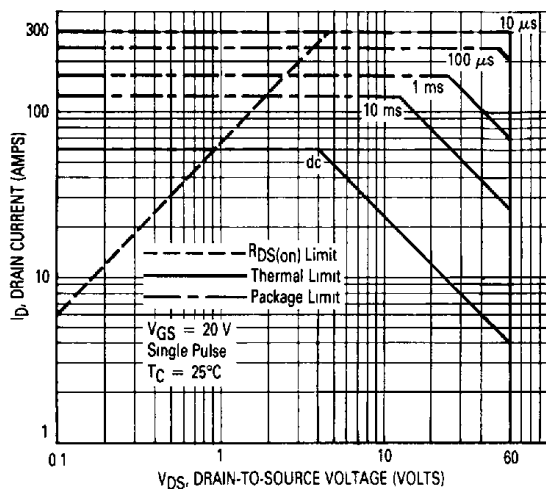
FIGURE 12 — MTM60N06
